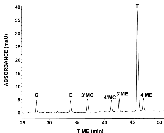
Fig. 2. High-performance liquid chromatogram of catechin (C), epicatechin (E), 3'-O-methyl-catechin (3'MC), 4'-O-methyl-catechin (4'MC), 3'-O-methyl-epicatechin (3'ME), 4'-O-methyl-epicatechin (4'ME) and taxifolin (T) with UV detection at 280 nm; 90 ng on-column.
