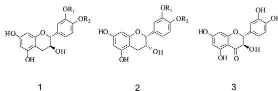
Fig. 1. Structures of (+)-catechin (1; R_1=H , R_2=H ), (-)-epicatechin (2; R_1=H , R_2=H ), 3'-O-methyl-(+)-catechin (1; R_1=CH_3 , R_2=H ), 4'-O-methyl-(+)-catechin (1; R_1=H , R_2=CH_3 ), 3'-O-methyl-(-)-epicatechin (2; R_1=CH_3 , R_2=H ), 4'-O-methyl-(-)-epicatechin (2; R_1=H , R_2=CH_3 ) and (+)-taxifolin (3).
