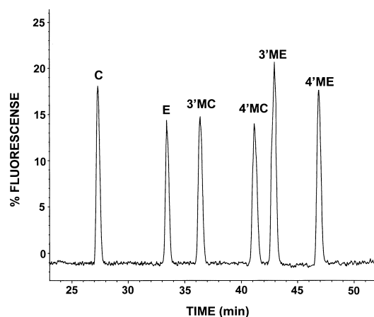
Fig. 3. High-performance liquid chromatogram of catechin (C), epicatechin (E), 3'-O-methyl-catechin (3'MC), 4'-O-methyl-catechin (4'MC), 3'-O-methyl-epicatechin (3'ME), 4'-O-methyl-epicatechin (4'ME) with FL detection, excitation at 280 nm and emission at 310 nm; 70 ng on-column.
